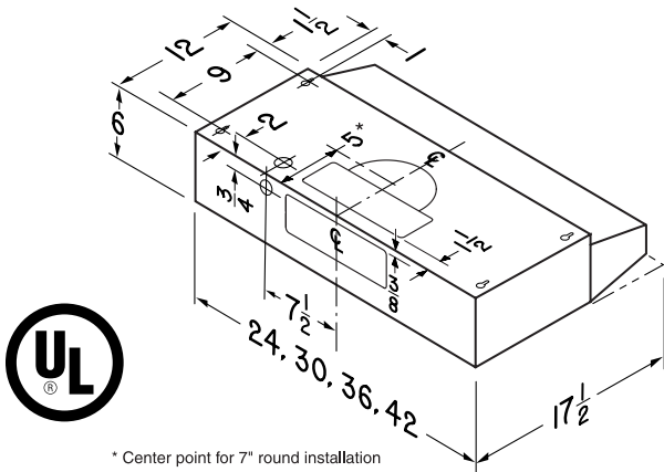
* Center point for 7" round installation
