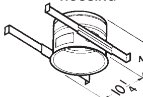
MODEL 504 HOUSING
