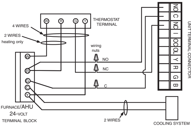
ALTERNATE FURNACE/AHU INTERLOCK WIRING
