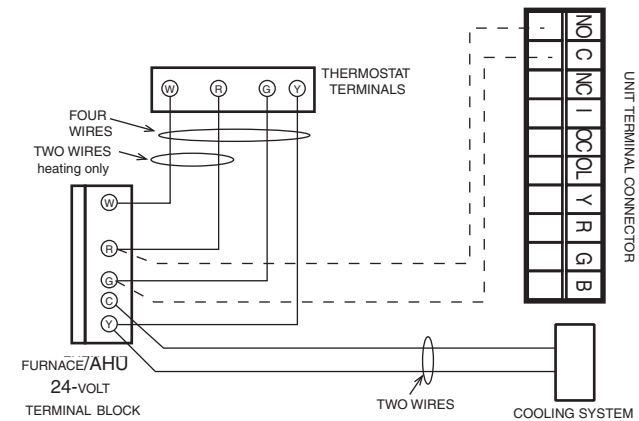
STANDARD FURNACE/AHU INTERLOCK WIRING
